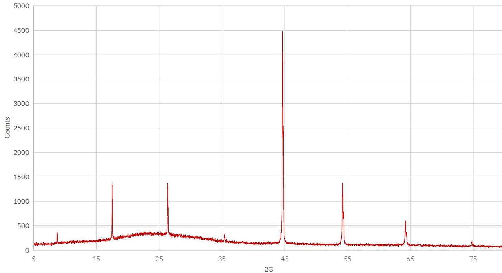
\text{Sb}_2\text{Te}_3 , XRD Spectrum (Batch 2017/001)
